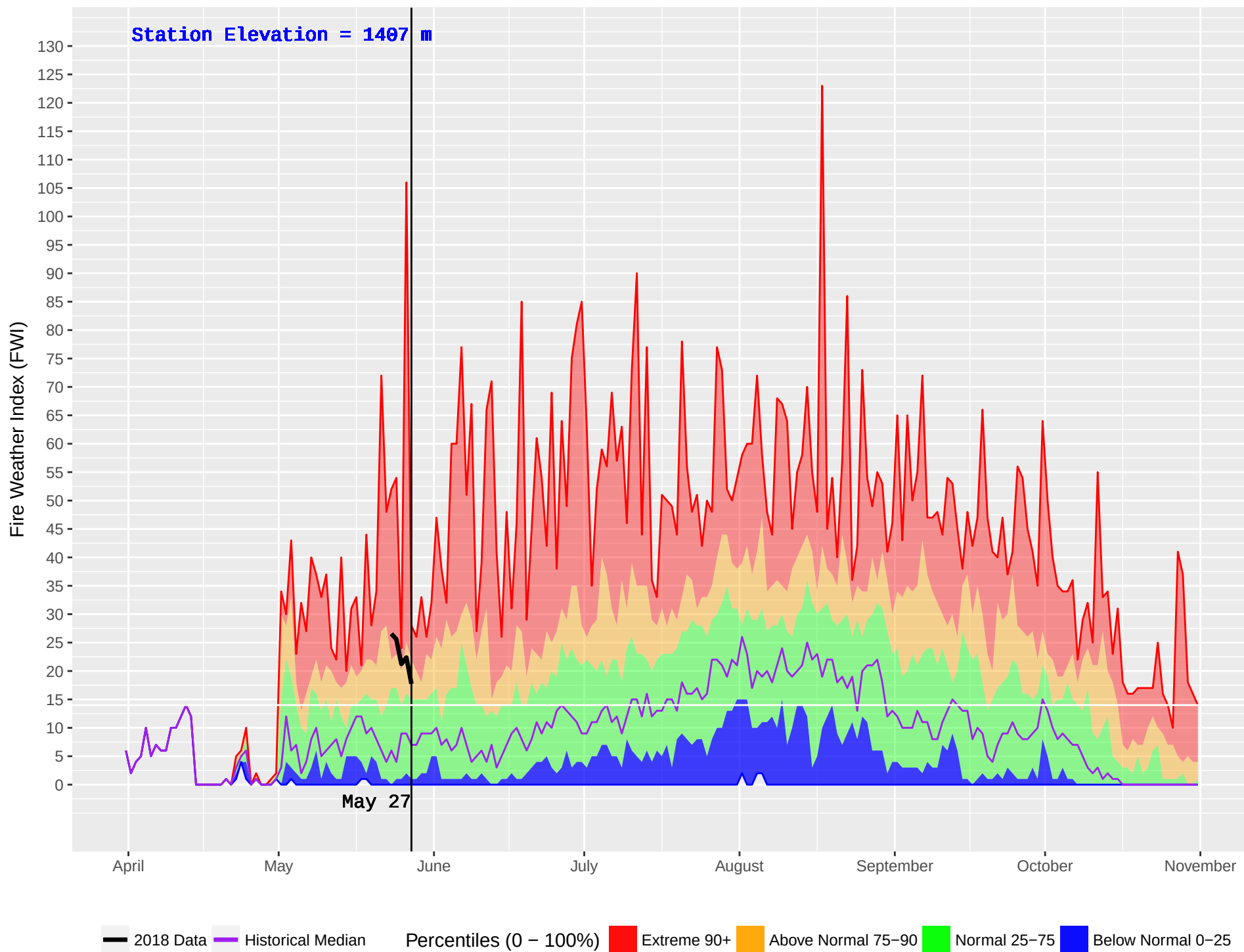
THYNNE (279) : Historical (1977–2016) and Current (2018) Noon Fire Weather Index (FWI)
