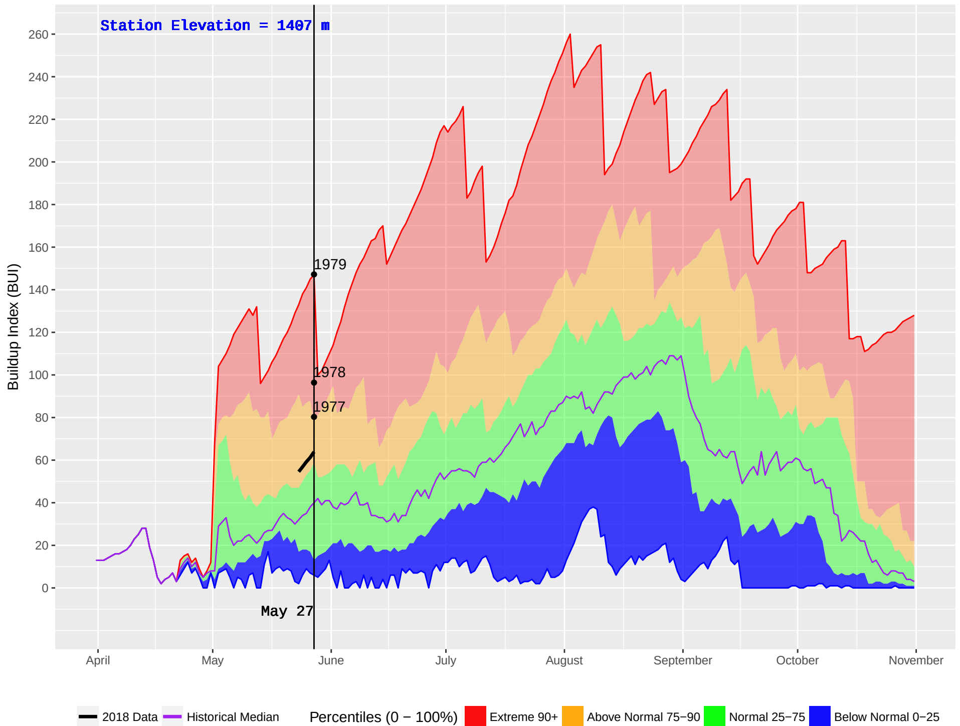
THYNNE (279) : Historical (1977–2016) and Current (2018) Noon Buildup Index (BUI)
